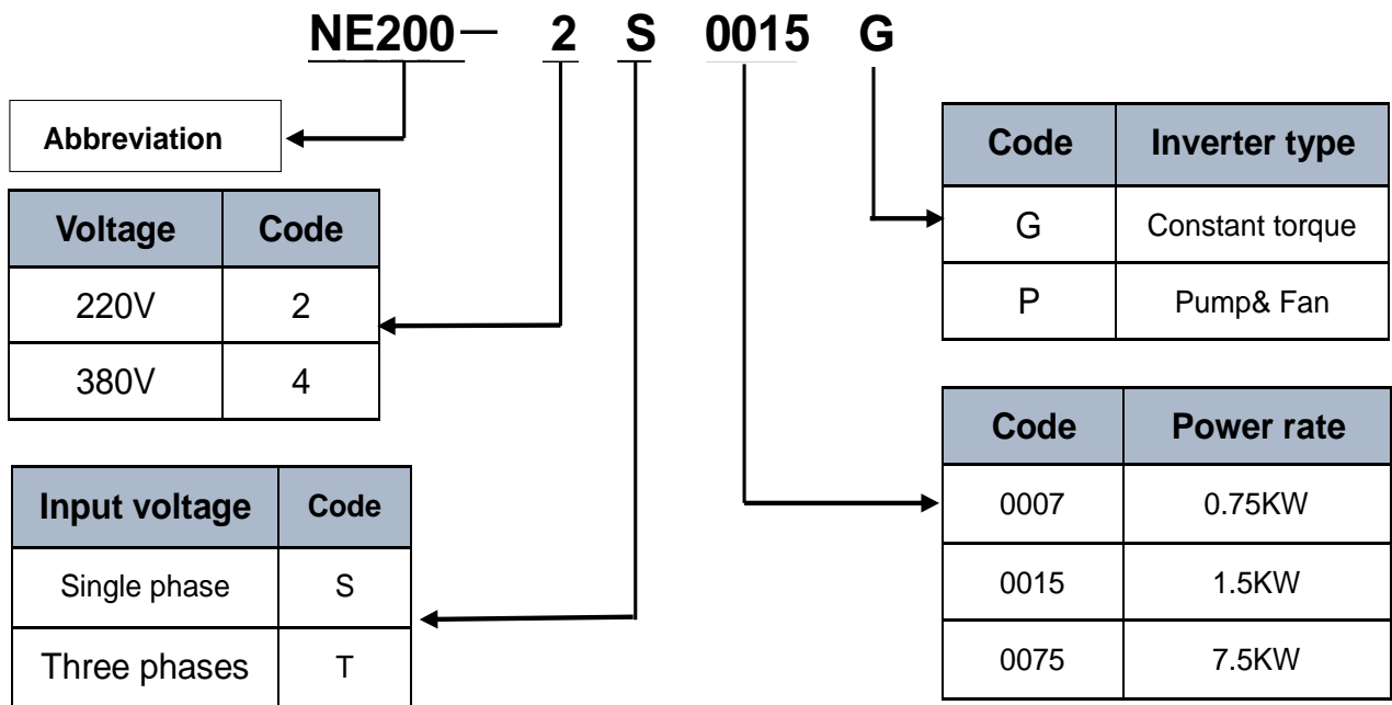
Fig 2-1 Inverter model description
